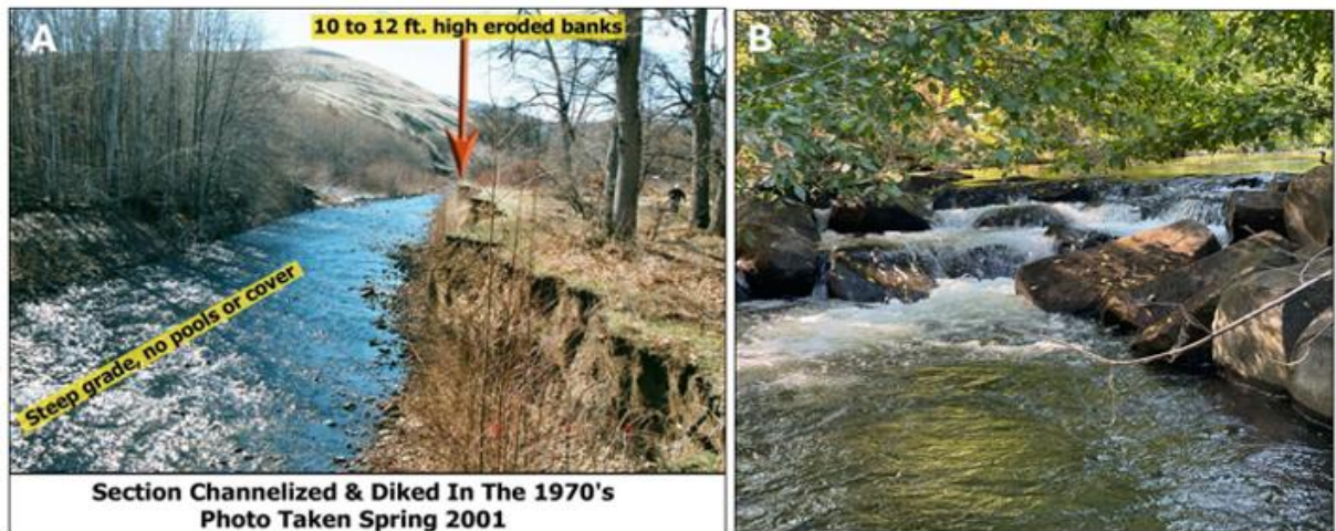
Figure 3. Photos of (A) Simplified channel confined against valley wall (from Reichmuth, 2007); (B) Example of one of the 15 boulder weir grade control structures built in 2000s
