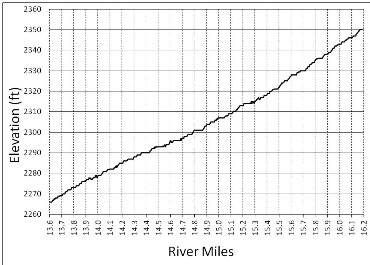
Figure 66. Longitudinal profile of Reach 5. Elevation data is derived from the 2006 LiDAR data and so represents water surface at the time of the LiDAR flight.
